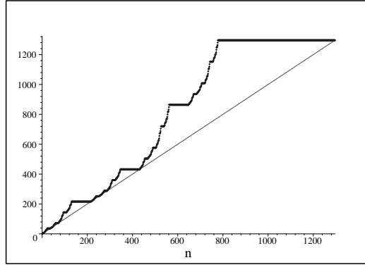
Figure 2: D_n ( n \leq 6^4 ) on the complete product of \mathcal{S}_3
