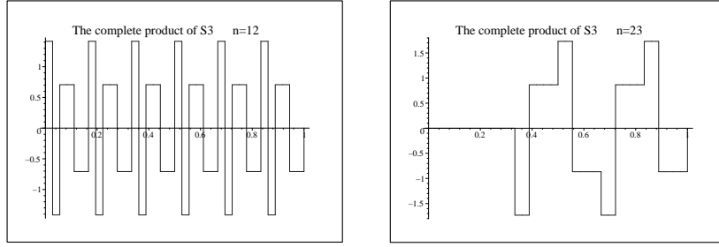
Figure 1: \psi_{12} and \psi_{23} with respect to the complete product of \mathcal{S}_3 .
